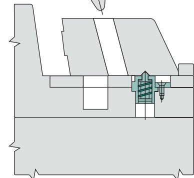
MOLD OPEN
